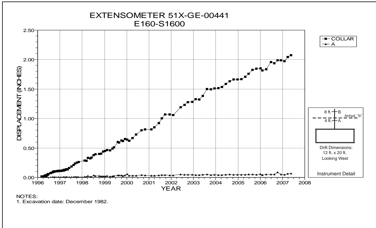
Figure 4-21 Extensometer 51X-GE-00441 S1600 Drift at E160 – Roof
